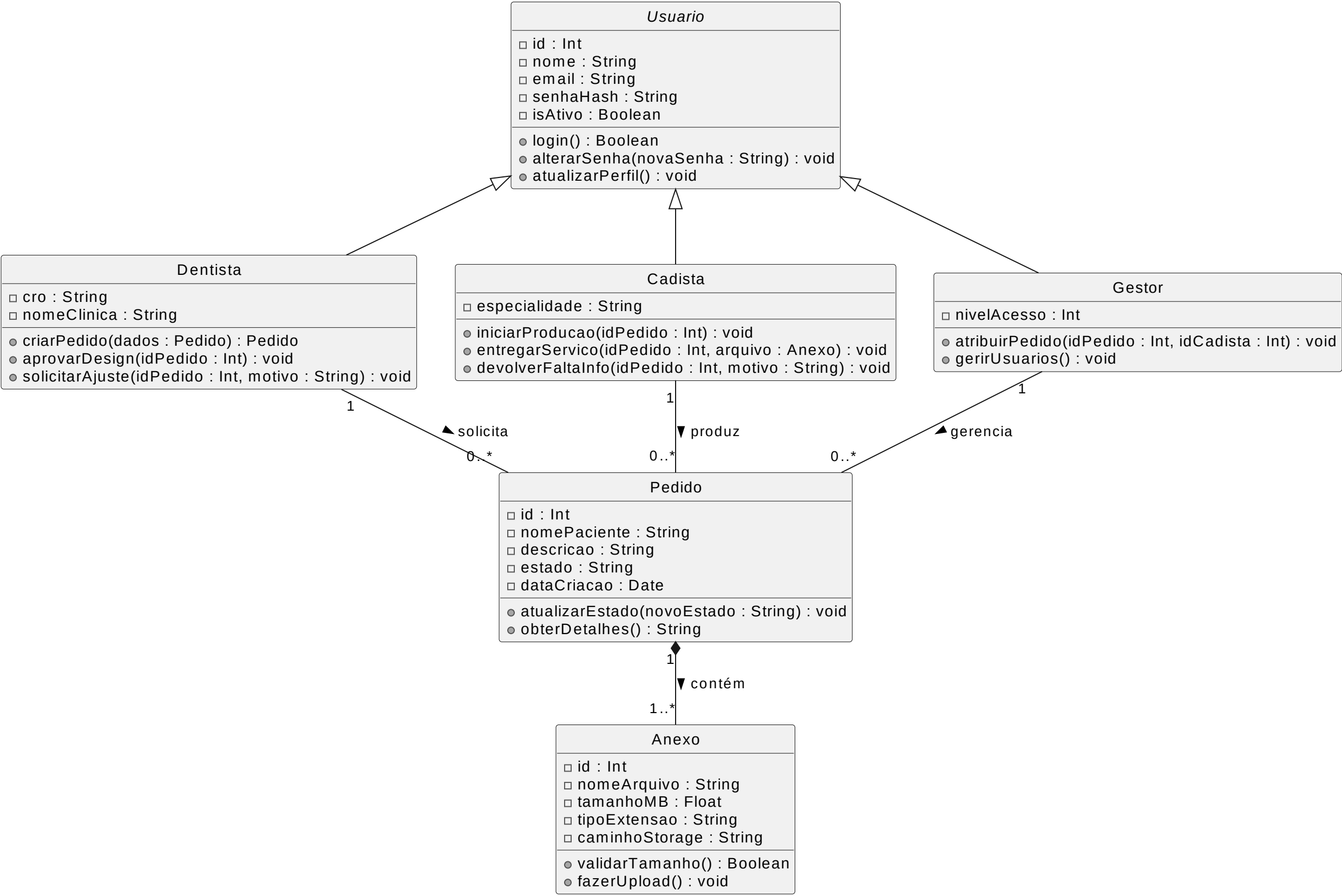
Diagrama de Classes UML: Protese Flow
